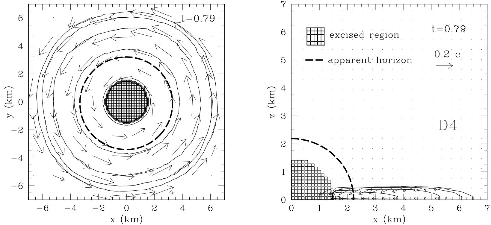
Figure 12: Time = 0.79 ms: the disc is unstable and is rapidly accreted onto the black hole.
