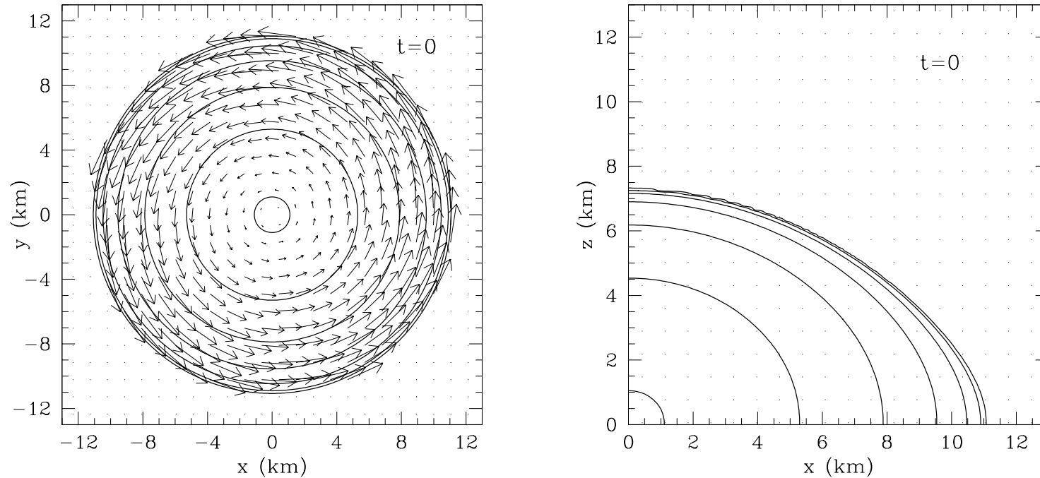
Figure 9: Collapse sequence for the rapidly rotating model D4. The conventions used in these panels are the same as in Fig. 5, which can be used for a comparison with the collapse of a slowly rotating model.
