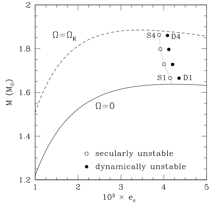
Figure 4: Gravitational mass shown as a function of the central energy density for equilibrium models constructed with the polytropic equation of state ( \Gamma = 2 , K_{\text{ID}} = 100 ). The solid, dashed and dotted lines correspond to the sequence of nonrotating models, the sequence of models rotating at the mass-shedding limit and the sequence of models that are at the onset of the secular instability to axisymmetric perturbations.
