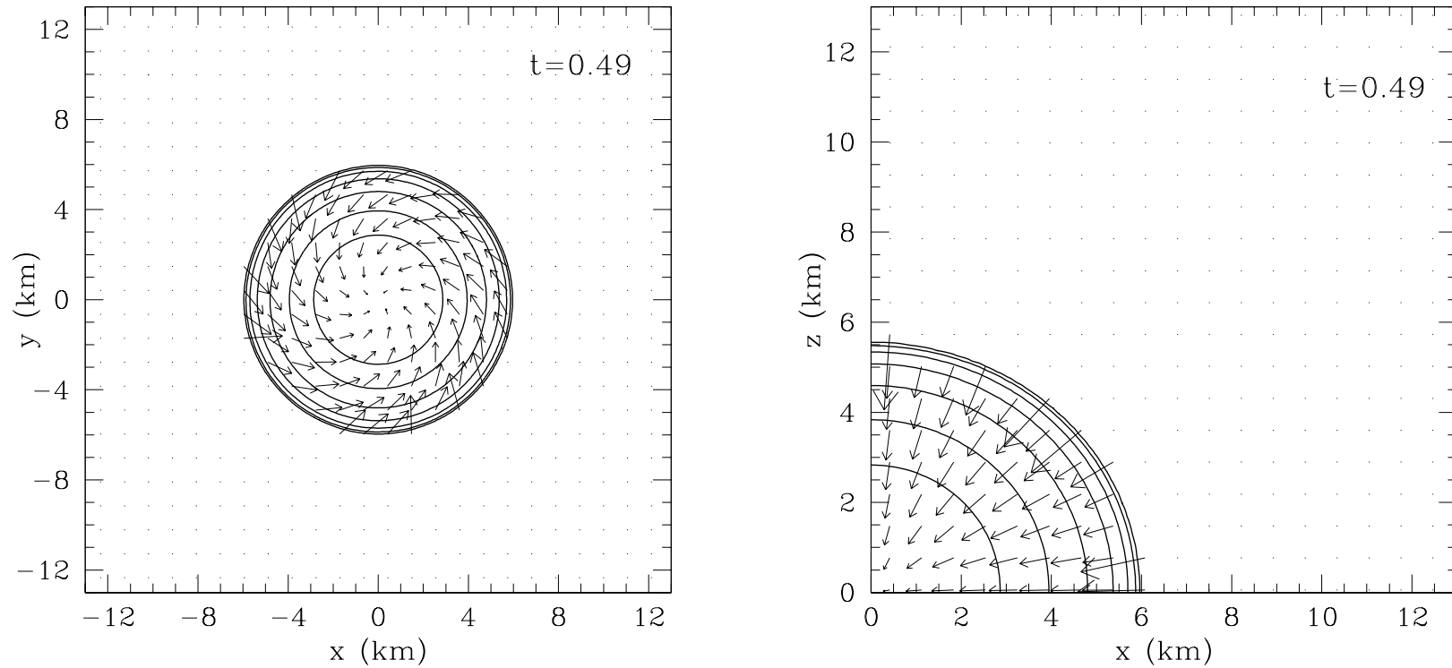
Figure 6: Time = 0.49 ms.
