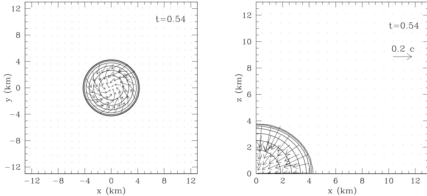
Figure 7: Time = 0.54 ms.
