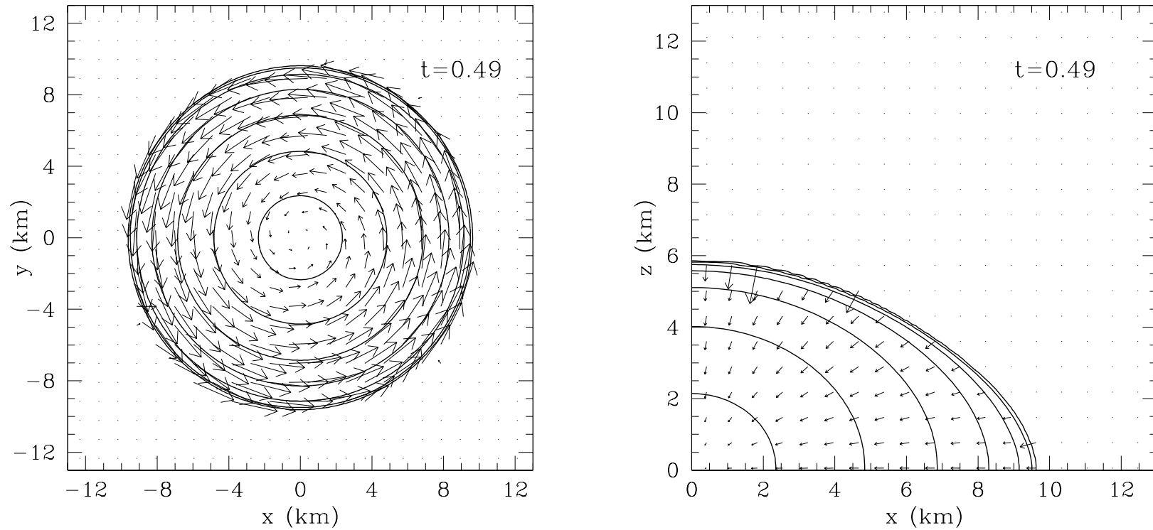
Figure 10: Time = 0.49 ms.
