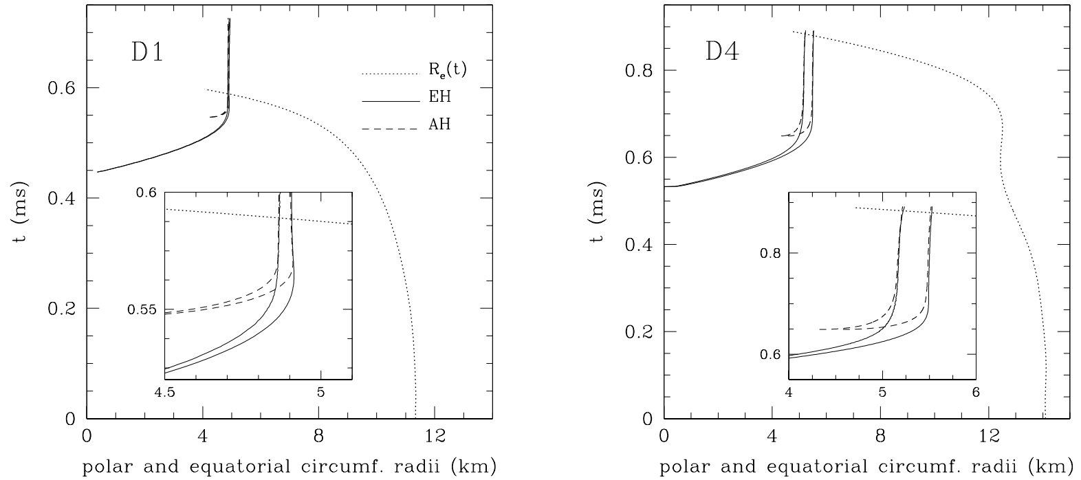
Figure 13: Solid, dashed and dotted lines represent the worldlines of the circumferential radii of the event horizon, of the apparent horizon and of the stellar surface, respectively. Note that for the horizons we plot both the equatorial and the polar circumferential radii.
