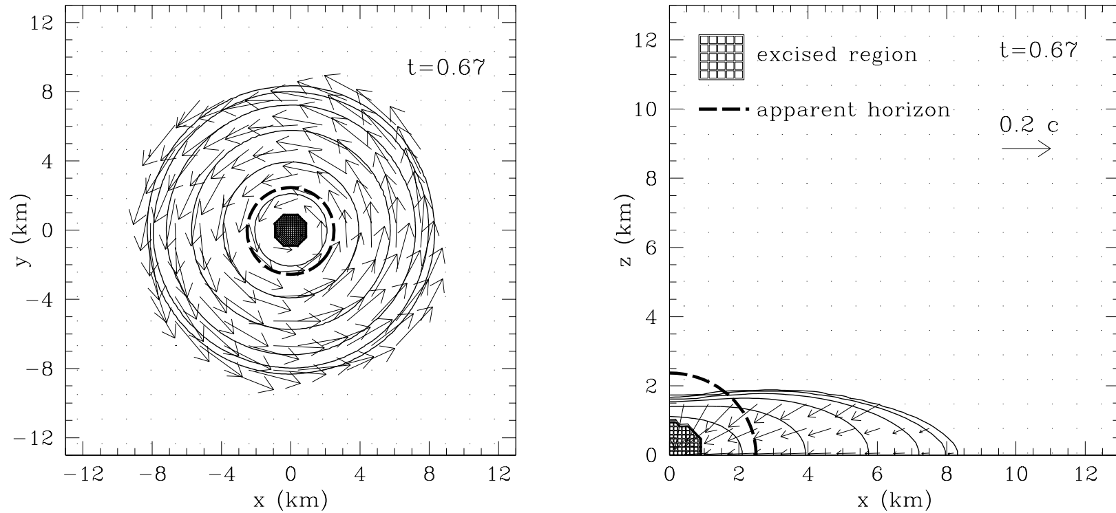
Figure 11: Time = 0.67 ms: an apparent horizon has just been formed.
