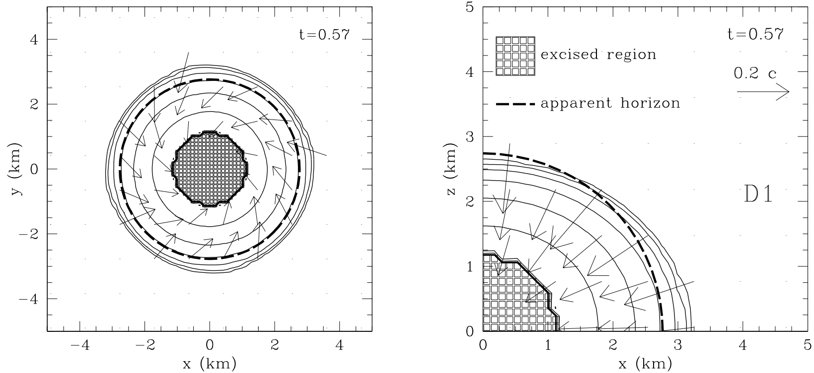
Figure 8: Time = 0.57 ms: an apparent horizon has just been formed.
