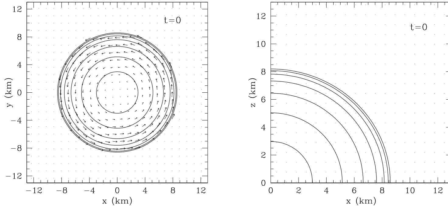
Figure 5: Collapse sequence for the slowly rotating model D1. Different panels refer to different snapshots during the collapse and show the isocontours of the rest-mass density and velocity field in the (x, y) plane (left column) and in the (x, z) plane (right column), respectively.
