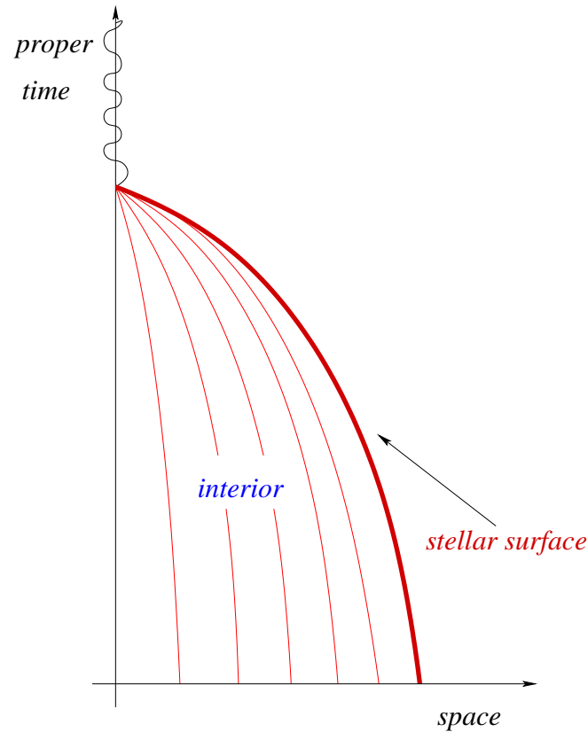
Figure 1: Schematic worldlines of dust shells in an OS collapse. Note that all the shells reach the singularity at the same proper time.
